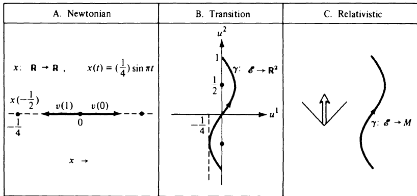
Figure 0.2.3. Three descriptions of motion in a straight line; note the simplicity of C.
