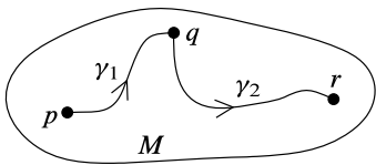
Fig. 13.2 The triangle inequality
