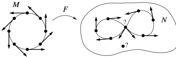
Fig. 8.2 The differential might not take vector fields to vector fields
