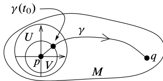
Fig. 13.3 Positivity of d_g
